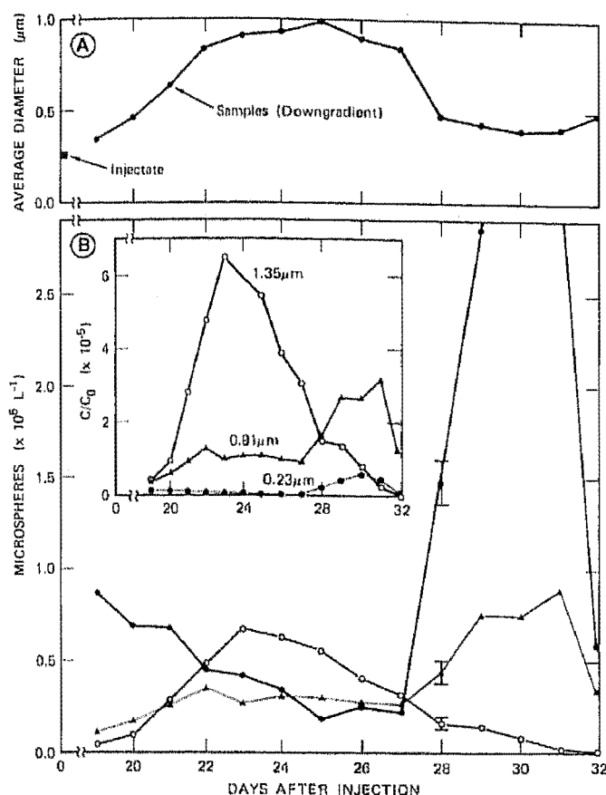
Figure 4. Average microsphere diameter (A) and concentration histories (B) for 0.23, 0.91, and 1.35- \mu\text{m} (diameter) carboxylated microspheres in the natural-gradient test. Dimensionless concentration history is depicted in the inset.
