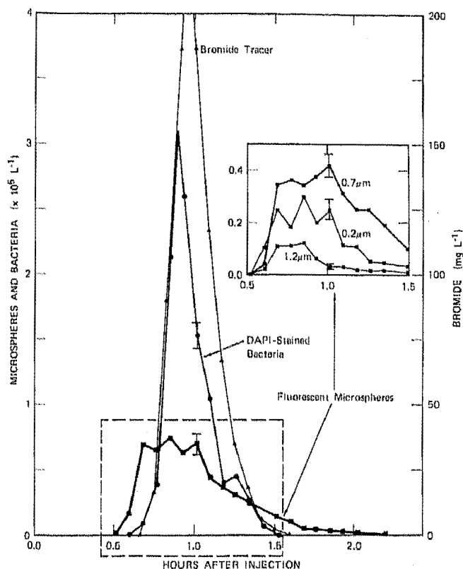
Figure 2. Concentration histories for bromide, DAPI-stained bacteria, and fluorescent microspheres (0.2, 0.7, and 1.2- \mu m diameter) at the closest sampler in the forced-gradient test.
