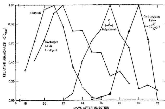
Figure 5. Concentration histories for chloride, uncharged latex (0.53- \mu\text{m} -diameter), polyacrolein (0.84- \mu\text{m} -diameter), and carboxylated latex (0.53- \mu\text{m} -diameter) microspheres in the natural-gradient test. Data have been normalized to maximum concentrations.
